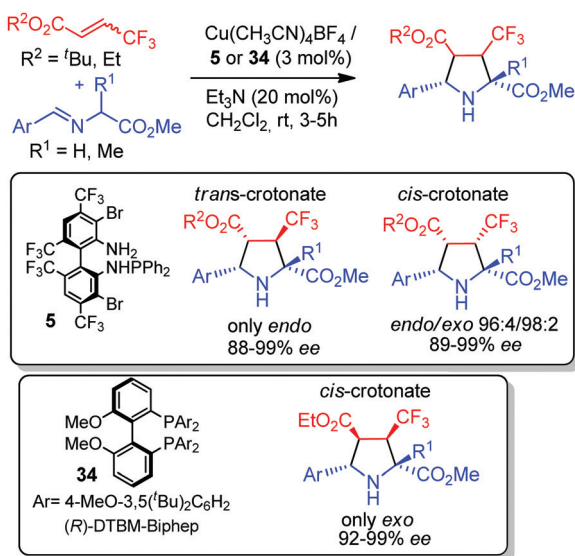
Scheme 15 \text{Cu}^I /( S )-TF-BiphamPhos catalyzed cycloaddition with trifluorocrotonates.
