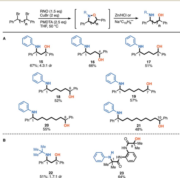
Fig. 2 Scope of amino-alcohols synthesized with a one-pot-two-step approach. (A) Products derived from benzyl dibromide scaffolds and nitrosobenzene. (B) Products derived from benzyl dibromide and the 2-methyl-2-nitrosopropane dimer or \alpha -bromocarbonyl compounds and nitroso benzene.
