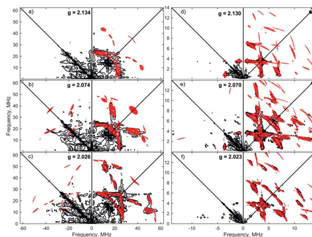
Fig. 5 X-band 4-pulse HYSCORE spectra of [\text{1} \cdot \text{H}_2]^+[\text{BAR}_4]^- (panels a–c) and [\text{1}(\text{H}_2)_2]^+[\text{BAR}_4]^- (panels d–f) at 2.5 mM in 7 : 1 PhMe : DFB, each collected at three field positions as indicated by g -value. The samples were frozen glasses at 20 K and measured with pulse lengths for ^2\text{H} of \pi/2 = 12 ns and \pi = 8 ns, \tau = 204 ns, initial variable delays of 100 ns and a time step of 20 ns over 300 points in both axes. The pulse lengths for ^1\text{H} were \pi/2 = 8 ns and \pi = 12 ns, \tau = 144, 140, 132 ns (top to bottom), initial variable delays of 100 ns and a time step of 8 ns, and 200 points in both axes. The microwave frequency was 9.7411 and 9.7583 GHz, respectively. Experimental data is in black, while simulations are overlaid in red.
