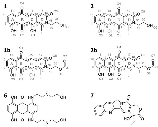
Fig. 6 Structures of the two pyxidicycline derivatives A ( 1 ) and B ( 2 ) as well as the corresponding formate esters ( 1b and 2b ) as determined by structure elucidation using NMR and X-ray crystallography. 6 and 7 , structures of mitoxantrone and camptothecin. 30,31
