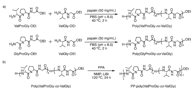
Scheme 2 (a) Chemoenzymatic copolymerization of Pro- and Val-containing di- and tri-peptides using papain and (b) post-polycondensation of poly(ValProGly-co-ValGly).
