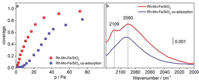
Fig. 7 Adsorption isotherms of CO adsorbed on Rh–Mn–Fe/SiO 2 determined using infrared spectroscopy at 77 K (without (red) and (blue) pre-adsorption of H 2 (a)), and FTIR spectra of adsorbed CO (coverage 10%) on Rh–Mn–Fe/SiO 2 at 77 K without (red) and with (blue) pre-adsorption of H 2 (b). The ratio of partial pressures of H 2 and CO corresponds to H 2 : CO = 3 : 1.
