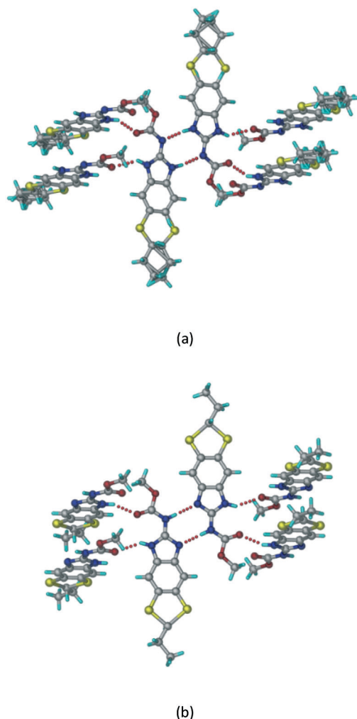
Fig. 1 ABZ crystal structures reported in the literature. ABZ exhibits sulphur attached alkyl disorder and the imidazole rings show tautomerism labelled as (a) form II (ref. 9) and (b) form I. 10 CSD ref codes SUTWIO, BOGFUZ.
