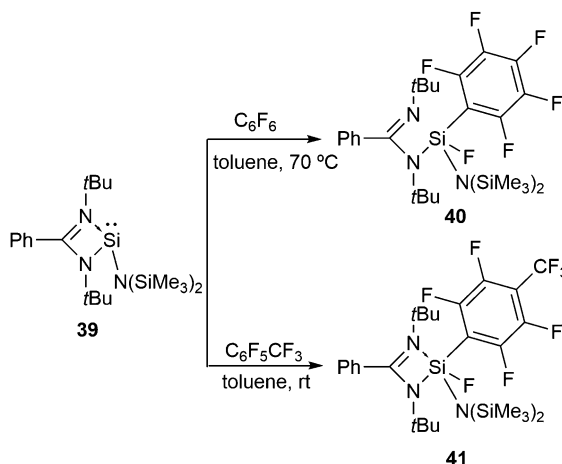
Scheme 14 \text{PhC}(\text{N}(\text{tBu})_2)\text{SiN}(\text{SiMe}_3)_2 mediated aromatic C–F bond activation.
