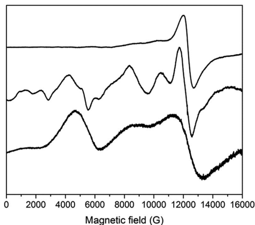
Fig. 8 Q-Band EPR spectra of powdered samples of (from top to bottom) [\text{FeL}_3]_2 , 2 and 1 at 5 K.
