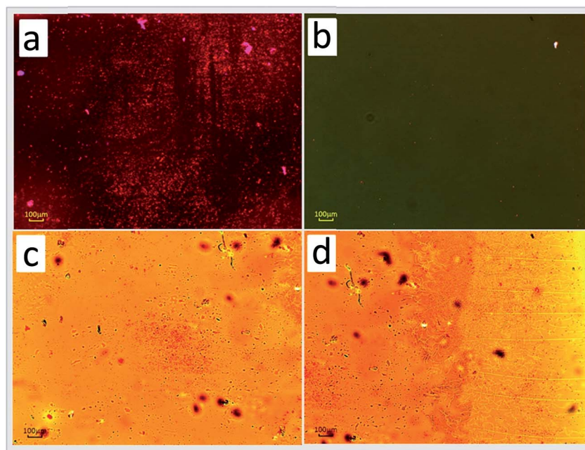
Fig. 9 Optical microscope photographs of (a) DCNP, (b) PY- o CNNO 2 and (c), (d) PY- p NO 2 compounds. The large (a, c) and small (b) groups of little crystals suspended in the polymeric layer are clearly seen. Layer cracks (d) are caused by the slow evaporation process of the solvent facilitating the nucleation and growth of microcrystals. Reprinted with permission from ref. 119. Copyright 2014 American Chemical Society.
