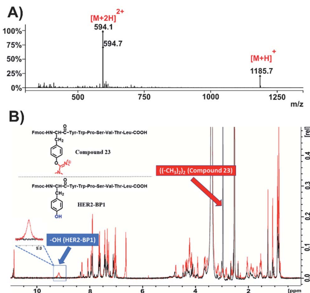
Fig. 4 Characterization of compound 23 . (A) ESI-MS spectrum of compound 23 ; (B) overlay of ^1\text{H} -NMR spectra of compound 23 (black color) and Fmoc-HER2-BP1 (red color) in \text{DMSO-d}_6 at 298 K.
