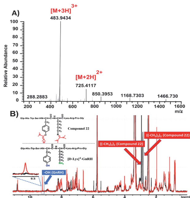
Fig. 3 Characterization of compound 22 . (A) HRMS spectrum of compound 22 ; (B) overlay of ^1\text{H} -NMR spectra of compound 22 (black color) and [D\text{-Lys}]^6\text{-GnRH} (red color) in \text{DMSO-d}_6 at 298 K.
