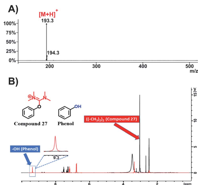
Fig. 8 Characterization of compound 27. (A) ESI-MS spectrum of compound 27; (B) overlay of ^1\text{H} -NMR spectra of compound 27 (black color) and phenol (red color) in DMSO- d_6 at 298 K.
