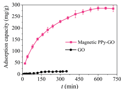
Fig. 11 Effect of time on the removal of Hg(II) with GO and magnetic PPy-GO. Conditions: T = 300 K, C_0 = 20 mg L ^{-1} , RSL = 0.05 g L ^{-1} and pH = 7.0 \pm 0.1 for magnetic PPy-GO; T = 298 K, RSL = 0.5 g L ^{-1} , C_0 = 100 mg L ^{-1} and pH = 6.0 for GO. 32
