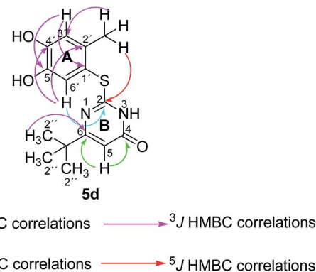
Fig. 5 Important 2 J, 3 J, 4 J and 5 J HMBC correlations of 5d .
