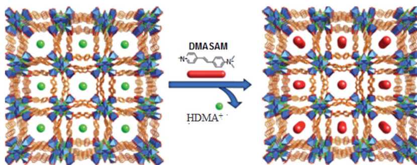
Fig. 17 Encapsulation of DMASM dye into (\text{Zn}_8(\text{Ad})_4(\text{BPDC})_6 \cdot 2\text{HDMA}) ( 99 ). Reproduced with permission from ref. 125, copyright 2013, Nature publish group.
