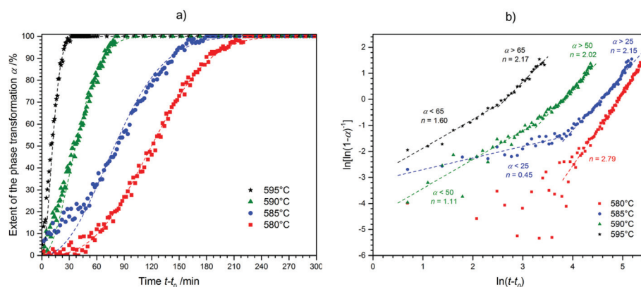
Fig. 5 (a) Progression of the phase fraction of \text{CsGaS}_2\text{-}m\text{C16} during the isothermal measurements (dashed lines indicate a fit based on the Avrami equation using the determined kinetic parameters n and K ). (b) Sharp–Hancock plots for the different experiments (dashed lines indicate a linear fit for the determination of n and K ).
