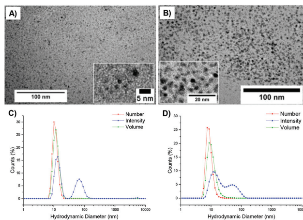
Fig. 3 Representative TEM images and size distributions, as determined by DLS (5 mg mL -1 in chloroform), of PEGA 98 - b -(DMAEA 76 -co-DEGDA 16 ), 2-20 (a and c), and PEGA 98 - b -(DMAEA 72 -co-DEGDA 8 ), 2-10 (b and d) prepared by arm-first RAFT polymerization.
