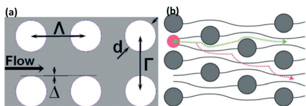
Fig. 9 Nanoparticles can be separated with a deterministic lateral displacement device. (A) Shows DLD design parameters, with d as pillar diameter, and l and \Delta as row and column periods, respectively, while \Delta is the shift fraction. Reproduced with permission from ref. 156 (B) Nanoparticles whose diameter is less than the critical diameter move in a zig-zag mode, while large particles cross the streamlines and displace laterally in bumping mode. Reproduced from ref. 158 with permission from The Royal Society of Chemistry.
