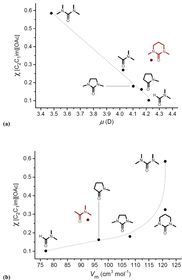
Fig. 6 Understanding the factors contributing to an effective OES solvent: relationship between minimum [C_2C_1im][OAc] mole fraction required for 10 wt% cellulose dissolution, \chi_{IL} , and the co-solvent dipole moment ( \mu ), (a), and molar volume ( V_m ), (b). Adapted with permission from J. Chem. Eng. Data , 2012, 57, 1341–1343. Copyright 2012 American Chemical Society.
