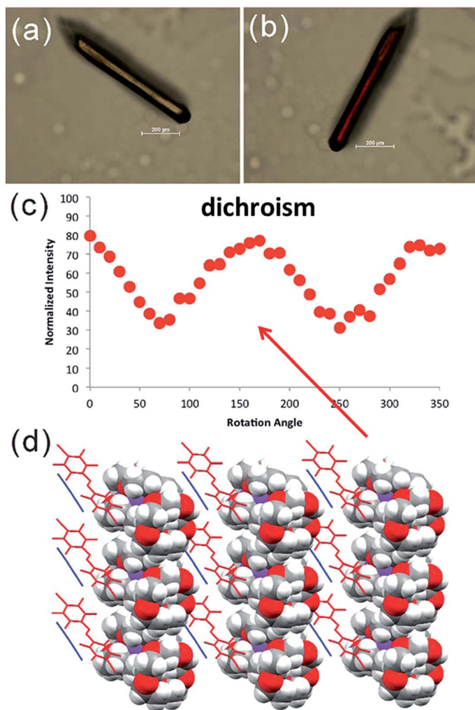
Fig. 17 Dichroic crystals of [\text{K}(15\text{-crown-5})][\text{Au}(\text{CN})_2] \cdot (\text{DIFAB}) \cdot (\text{solvent}) ( \text{DIFAB} = 4,4' -diiodooctafluoroazobenzene) containing aligned linear halogen-bonded assemblies of DIFAB and [\text{Au}(\text{CN})_2]^- . (a) and (b) Crystals presented at different rotation angles exhibit different colours in polarised light. (c) Light intensity as a function of crystal rotation. (d) Crystal structure [\text{K}(15\text{-crown-5})][\text{Au}(\text{CN})_2] \cdot (\text{DIFAB}) \cdot (\text{solvent}) . Reproduced from DOI: 10.1039/c7fd00114b with permission from The Royal Society of Chemistry.
