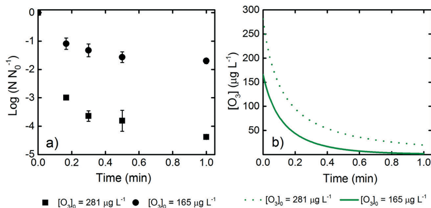
Fig. 7 At 22 °C (a) the effect of HRT on L. pneumophila inactivation, at two initial ozone concentrations and a WOM loading of 3.1 mg C L^{-1} in a semi-batch reactor; (b) the profile of two initial dissolved ozone concentrations as a function of HRT. The data plotted in (a) are average values and standard deviations of three replicates. The dashed and solid curves in (b) are the results of calculations.
