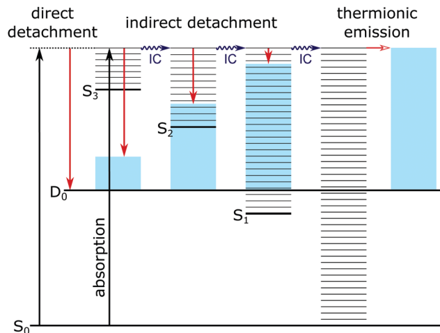
Fig. 4 Jablonski diagram illustrating the major photodetachment pathways (red arrows) available for the model PYP chromophores employed in this work (Fig. 2) following UV photoexcitation (346–310 nm) including internal conversion (IC) and thermionic emission (horizontal red arrow). Horizontal black lines represent the vibrational levels of the excited electronic states of the anion and the blue shaded areas represent the vibrational energy left in the neutral radical upon electron detachment as a result of the propensity for conserving vibrational energy.
