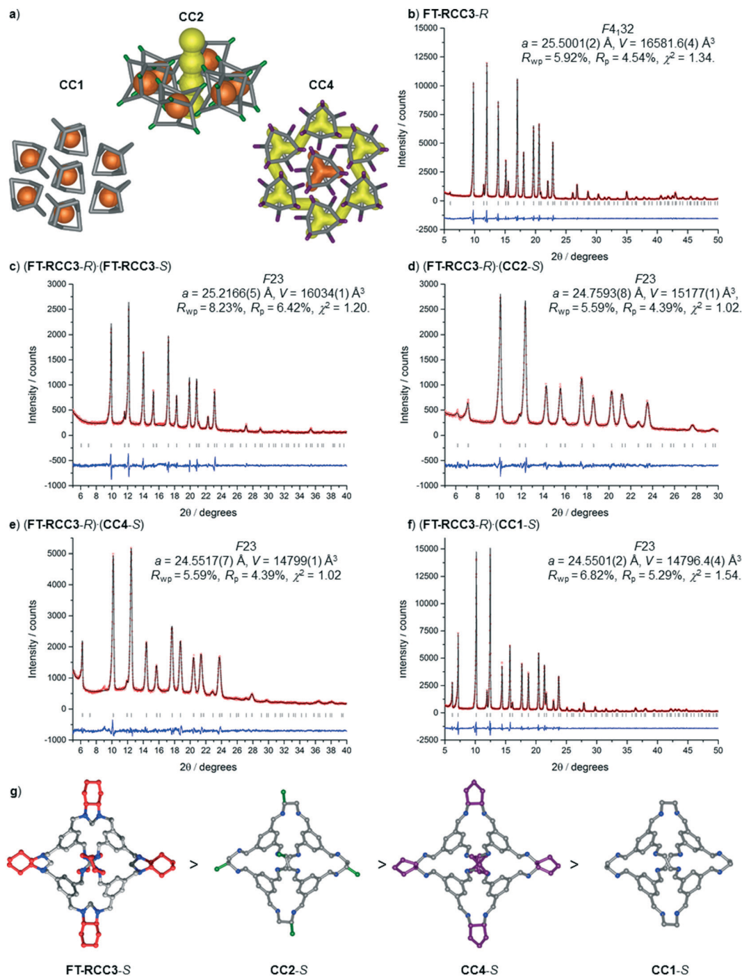
Fig. 5 (a) Graphical representation of pore networks in most commonly observed crystal structures for CC1, CC2-R and CC4-R. Le Bail fit's for PXRD refined data, (b) FT-RCC3-R, (c) racemic FT-RCC3, (d) (FT-RCC3-R)-(CC2-S), (e) (FT-RCC3-R)-(CC4-S), and (f) (FT-RCC3-R)-(CC1-S); shown in order or decreasing unit cell volume (b \rightarrow f) that correlates with the trend shown in (g) when these -S handed cages are co-crystallised with FT-RCC3-R.
