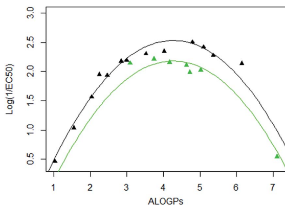
Fig. 6 lmer fit and model for the alkyl R type, OMe ring substituent (coefficients for ALOGPs and ALOGPs-sq are fitted using all data-points). Points coloured by enamine-substituent: black – NH, green – NH-Ph.
