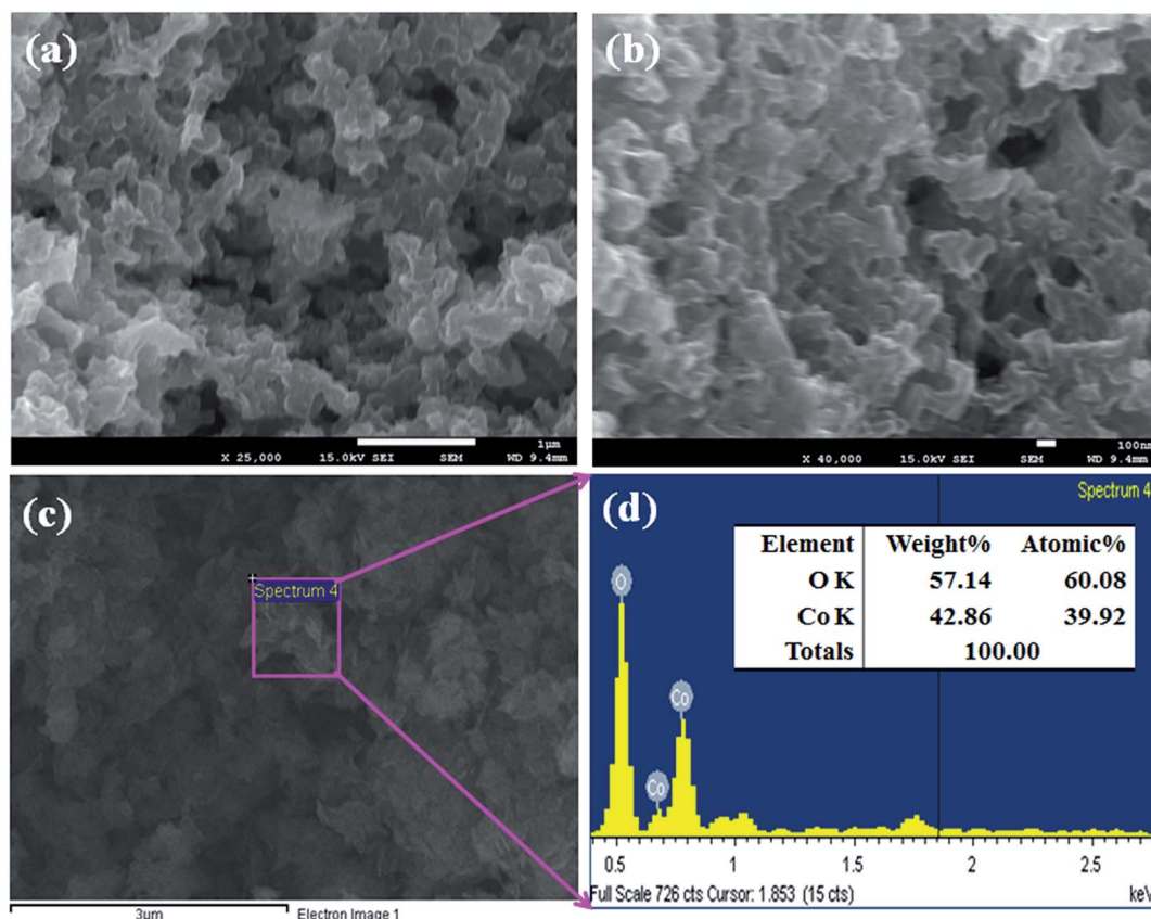
Fig. 2 (a and b) Low and high magnified images and (c and d) elemental analysis of the \text{Co}_3\text{O}_4 NSs.
