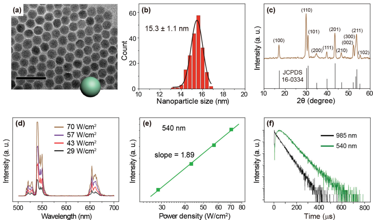
Fig. 2 (a) A typical TEM image of the as-prepared \text{NaYF}_4:\text{Yb}/\text{Er} (20/2%) nanoparticles. Scale bar is 50 nm. (b) Size histogram of the nanoparticles. (c) X-ray diffraction patterns of the nanoparticles, which are in good agreement with the literature reference for hexagonal \text{NaYF}_4 crystal (Joint Committee on Powder Diffraction Standards file number 16-0334). (d) Emission spectra of the UCNPs recorded with a 975 nm CW laser excitation at different power densities ( 29\text{--}70\text{ W cm}^{-2} ). (e) The 540 nm ( ^4\text{S}_{3/2} \rightarrow ^4\text{I}_{15/2} transition of \text{Er}^{3+} ) emission intensity versus pump power density in double-logarithmic representation. (f) Decay curves of 540 nm emissions from \text{Er}^{3+} as well as 985 nm from \text{Yb}^{3+} obtained upon excitation of the nanoparticles at 975 nm.
