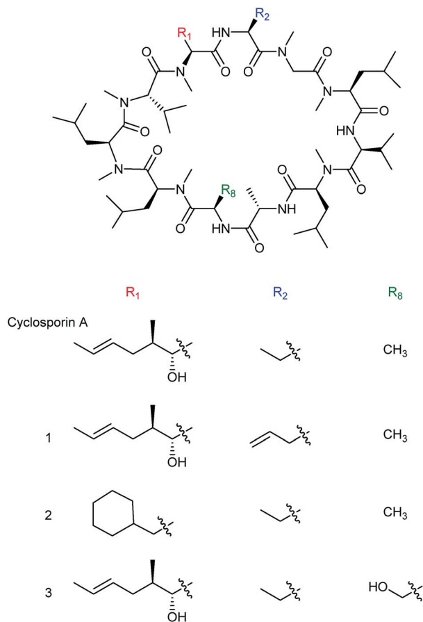
Fig. 3 Cyclosporin analogues incorporating nonnatural allyllysine (1), \beta -cyclohexylalanine (2) or D-serine residues (3) produced by precursor directed biosynthesis. 16
