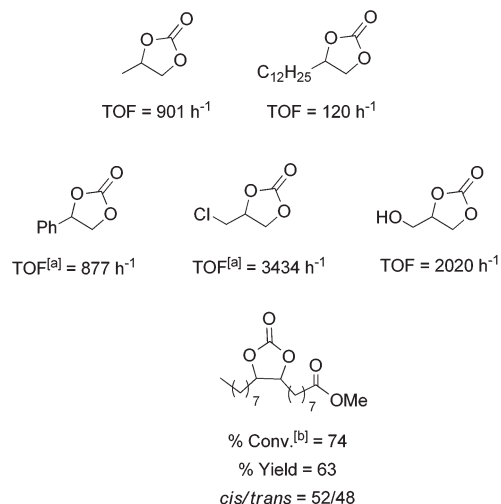
Fig. 5 Cycloaddition of different epoxides to CO 2 with the catalytic system 1 /TBAB. Reaction conditions: T = 80^\circ\text{C} , time = 0.5 h, P_{\text{CO}_2} = 10 bar, substrate: 3 ml; 1 : 0.05 mol%, TBAB: 0.25 mol%. a 1 : 0.03 mol%; TBAB: 0.15 mol; b 1 : 2 mol%, TBAB: 2 mol%; T = 100^\circ\text{C} ; P_{\text{CO}_2} = 100 bar. Reactions were run in duplicate.
