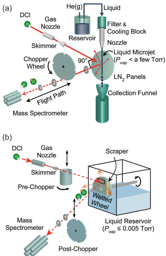
Fig. 3 Experimental setups used in our laboratory for molecular beam scattering experiments with (a) liquid microjets and (b) flat liquid films. The figure illustrates collisions of \text{DCI} that exit the liquids as \text{DCI} and \text{D} \rightarrow \text{H} exchanged \text{HCl} .
