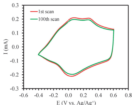
Fig. 5 Cyclic voltammograms of P(ProDOT-diene) film: 1st and 100th cycle is plotted.
