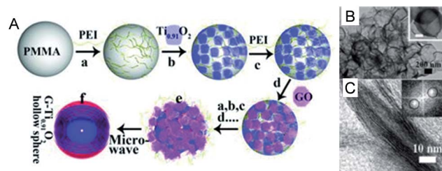
Fig. 23 (A) Stepwise preparation of alternating \text{TiO}_2 and graphene nanosheet hollow sphere assemblies, (B) TEM and (C) and HR-TEM images of (\text{G}-\text{Ti}_{0.91}\text{O}_2)_5 hollow spheres. Scale bar of the inset in (c): 100 nm. Inset in (C) is the fast Fourier Transform pattern of the ordered lamellar structures exhibited by the (\text{G}-\text{Ti}_{0.91}\text{O}_2)_5 hollow spheres. Reproduced with permission from ref. 210. Copyright 2012 Wiley.
