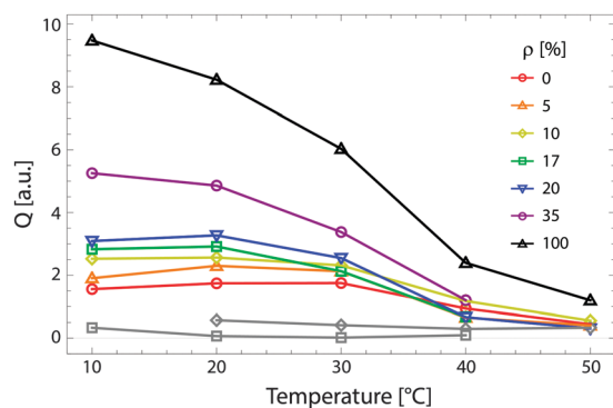
Fig. 9 Experimentally measured total scattering reveals domain formation in 4-component lipid mixtures. Shown is the Porod invariant Q = \int I(q) q^2 dq , plotted vs. temperature for DSPC/(DOPC + POPC)/Chol mixtures in a 0.39/0.39/0.22 molar ratio. Colors correspond to different values of the composition parameter \rho = \chi_{\text{DOPC}}/(\chi_{\text{DOPC}} + \chi_{\text{POPC}}) as indicated in the legend. Also shown are two single-phase control samples: DSPC/POPC/Chol 0.325/0.325/0.35 (gray diamond) and POPC/Chol 0.65/0.35 (gray square). Figure adapted from ref. 102.
