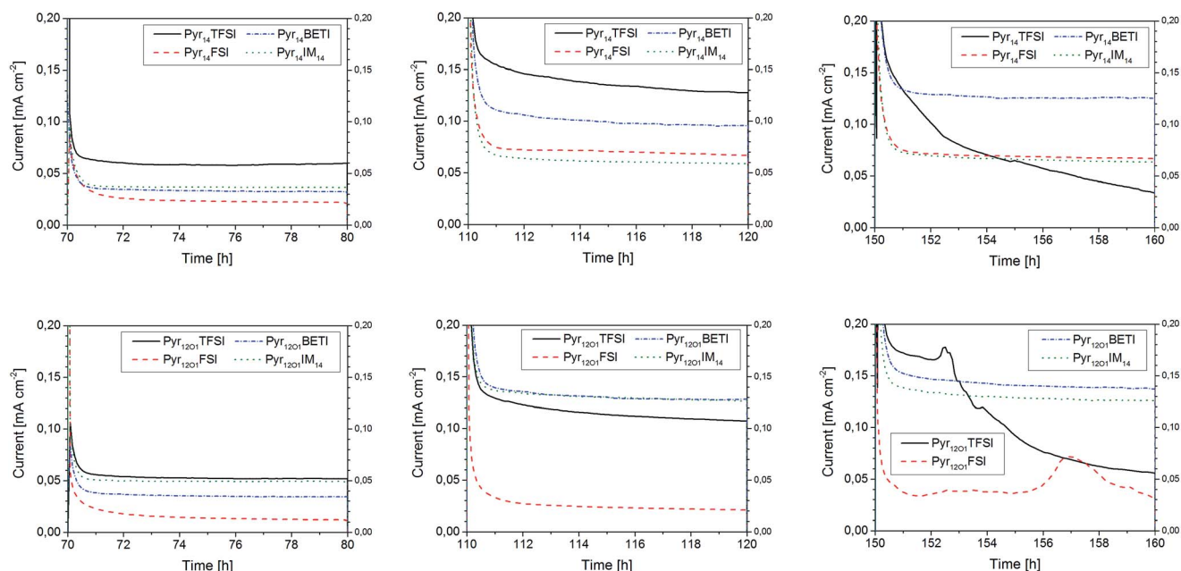
Fig. 7 Chronoamperometry curves upon 10 h polarization steps (intermixed with 10 h relaxation steps) at 0.2 V (left), 0.6 V (center) and 1.0 V (right); Pyr 14 -containing electrolytes (top) and Pyr 1201 -containing electrolytes (bottom). All measurements were performed at 40 °C.
