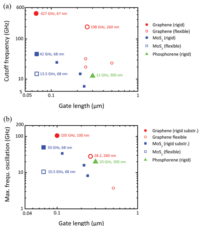
Fig. 13 RF performance of 2D MOSFETs on flexible and rigid substrates. (a) Cutoff frequency f_T vs. gate length. (b) Maximum frequency of oscillation f_{\max} vs. gate length. The respective record f_T and f_{\max} data are shown by large symbols. The numbers next to the record data points are the frequency ( f_T or f_{\max} ) and the gate length of the transistor. Data taken from ref. 179, 182, 187, 201, 205 and 206 for MOSFETs with graphene, from ref. 163 and 207 with MoS 2 , and from ref. 208 with phosphorene channels.
