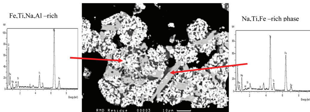
Fig. 9 The microstructure (10 μm) of porous insoluble residues left after alkali roasting of bauxite and red mud at 775 °C in air and leaching with hot distilled water above 50 °C. Time of roasting – 2 hours.
