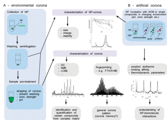
Fig. 11 Suggested experimental approach for investigating the environmental corona. (A) Characterization of environmental corona includes the determination of key properties, such as size and surface charge of corona covered NPs and NPs' after corona stripping. The subsequent identification and quantification of corona biomolecule components or comprehensive fingerprint analysis is depicted. (B) Creating an artificial model corona using selected representative NOM molecules (single substances) and determination of their dynamic adsorption behaviour as well as the influence of corona formation on NP properties ( e.g. size and surface charge) will assist model building and predictions.
