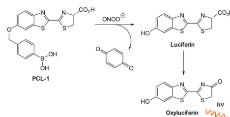
Fig. 81 Structure and reaction of luciferin based probe PCL-1 with ONOO - .
