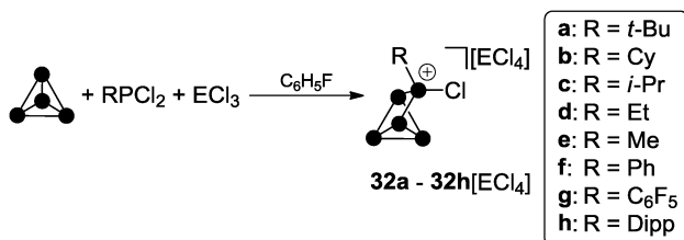
Scheme 8 Preparation of compounds 32a-h[\text{ECln}] from \text{P}_4 , \text{RnPCln} and \text{ECln}_3 (E = Ga, Al; R = alkyl, aryl) in fluorobenzene.
