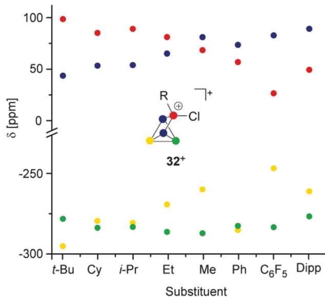
Fig. 8 Plot of the ^{31}\text{P} NMR chemical shifts of \text{RP}_5\text{Cl}^+ -cages 32a-h^+ versus their alkyl- or aryl-substituent.
