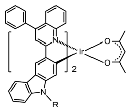
211: R = ethyl
