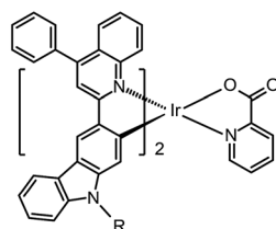
209: R = ethyl
