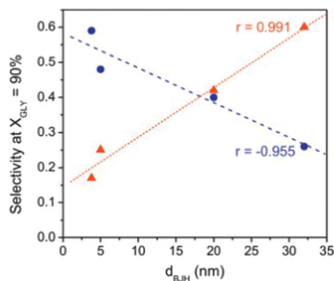
Fig. 14 Correlations between selectivities to dihydroxyacetone (DIHA – \blacktriangle ) and glyceric acid (GLYCEA – \bullet ) and the main pores size (calculated by the BJH method) for Au nanoparticles supported on mesoporous carbon supports. Reprinted with permission from ref. 144. Copyright 2012, Elsevier.
