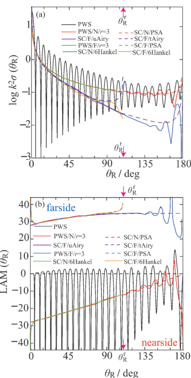
Fig. 4 Nearside–farside analyses for the dimensionless logarithmic angular distribution and the Local Angular Momentum. Black solid curve: PWS. Red solid curve: PWS/N/ r = 3 . Red dashed curve: SC/N/PSA. Solid purple curve: SC/F/uAiry. Purple dashed curve: SC/F/tAiry. Blue solid curve: PWS/F/ r = 3 . Blue dashed curve: SC/F/PSA. Green solid curve: SC/N/6Hankel. Orange solid curve: SC/F/6Hankel. The pink solid arrows indicate the rainbow angle, \theta_R^r = 109.2^\circ . (a) Full and NF \log k^2\sigma(\theta_R) versus \theta_R . (b) Full and NF \text{LAM}(\theta_R) versus \theta_R .
