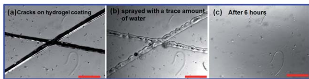
Fig. 5 The use of a dried self-healing hydrogel film as a protective coating. (a) A hydrogel coating with a crack of about 100 \mu\text{m} on a glass surface. (b) The hydrogel was sprayed with a trace amount of water. (c) The cracks self-healed completely after 6 hours. The scale bar is 500 \mu\text{m} .
