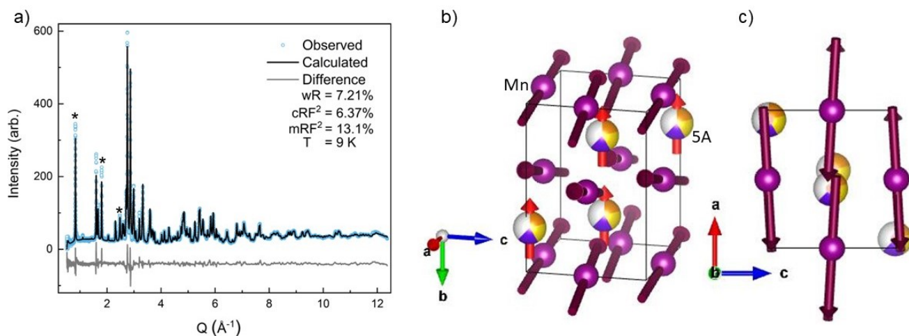
Fig. 5 (a) The 9 K magnetic and crystallographic refinement is shown with the difference curve, ( Data – Fit ) shifted down for visibility, in light gray. We obtained a good fit to the observed reflections with a wR of 7.21% for the whole fit and the crystallographic main phase obtaining a RF^2 of 6.37%, an RF^2 of 13.1% is obtained for the magnetic cif. The three main magnetic peaks are shown with *. (b) the magnetic CIF at 9 K is shown with the B-site Mn ions being purple and the A-site (5A) ions, showing the 60% occupancy with only Pr^{3+} , Nd^{3+} , and Tb^{3+} taking part in the magnetic structure. (c) View down the b -axis of the magnetic CIF.
