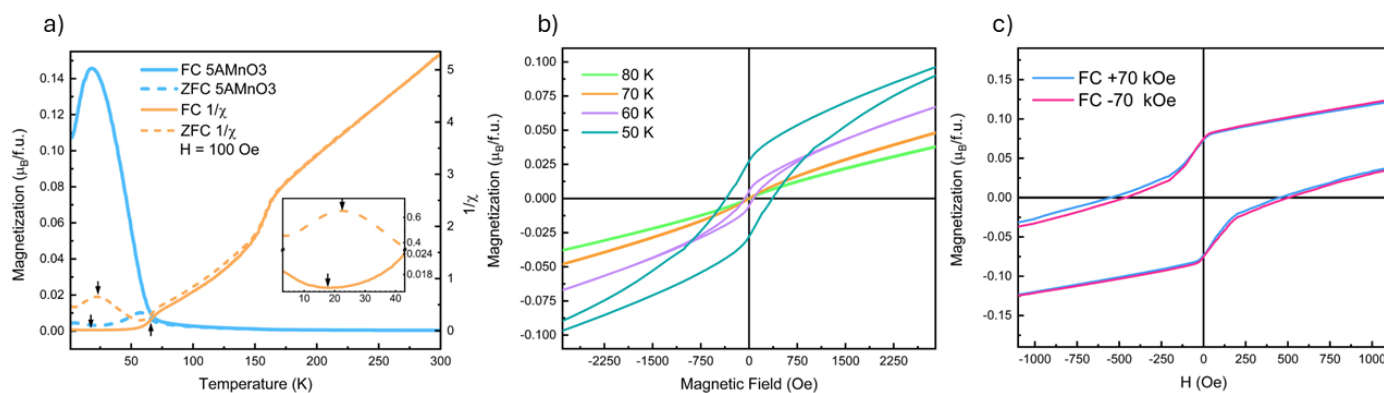
Fig. 2 (a) Magnetization versus temperature measured under a 100Oe applied field plotted with the inverse susceptibility, 1/\chi of the ZFC and FC MvT. Arrows have been placed at the inflections of the ZFC and FC 1/\chi plots to highlight the ordering temperatures of the A- and B-site sub-lattices with the inset of the figure showing the inflection points that correspond to the A-site ordering with a vertical axis break with differing y-axis scale on either side to allow the reader to see the inflection in both measurements. (b) Magnetization versus applied field taken around the magnetic transition at 67 K showing the opening of a hysteresis loop with cooling. (c) Magnetic exchange bias measurements ( \pm 70 kOe FC MvH) at 10 K showing the presence of pinning and an exchange bias. The main plot (c) has had the pinning removed to highlight the small exchange bias; the inset in (c) is the same data and scale before pinning subtraction.
