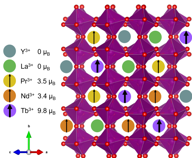
Fig. 1 Cartoon depiction of the (5A)\text{MnO}_3 unit cell showcasing the large variance in magnetic moment 17 on the A-site.
