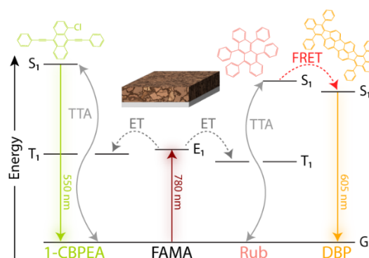
Figure 2: Energy flow schematic for UC process in the bilayer devices with the corresponding chemical structures for the OSC molecules. Incident 780 nm photons are absorbed by the perovskite, where charge transfer (ET) populates the triplet state T_1 of 1-CBPEA (left) or Rub (right). Interaction of two triplet states results in TTA, yielding the higher energy S_1 state. For Rub, an additional energy transfer (FRET) occurs to the DBP S_1 energy level. Resulting UC emission wavelengths are 550 nm for 1-CBPEA and 605 nm for RubDBP.
