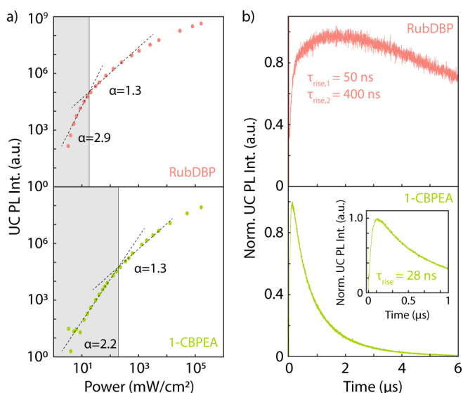
Figure 5: a) Power dependent upconverted emission for the RubDBP (top, pink) and 1-CBPEA (bottom, green) bilayer devices. The intersect of the dashed lines indicating the different TTA-UC regimes yields the I_{th} (vertical grey lines). Calculated intensity threshold I_{th} values for RubDBP and 1-CBPEA films are 18.2 \text{ mW cm}^{-2} and 195 \text{ mW cm}^{-2} , respectively. b) UC PL dynamics for the RubDBP (top) and 1-CBPEA (bottom) films (repetition rate: 50 kHz, power density: 120 \text{ mW cm}^{-2} ). A magnification of the early time rise for 1-CBPEA is shown in the inset.
