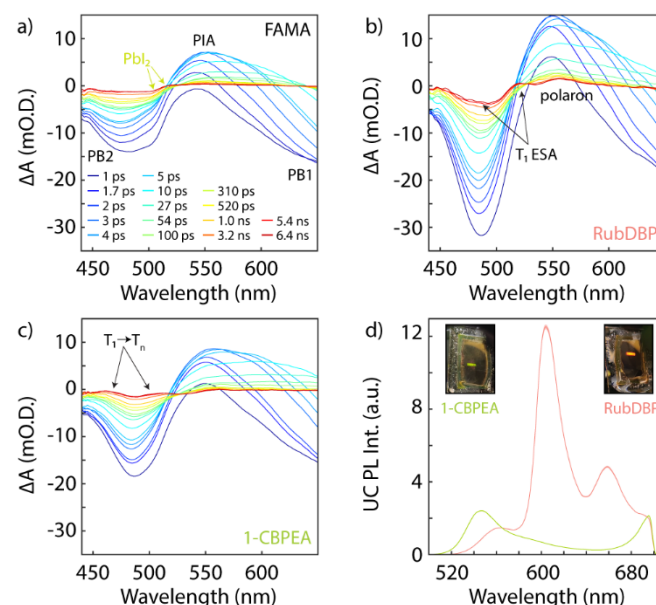
Figure 4: Absorbance spectra at selected delay times for a) FAMA, b) RubDBP, and c) 1-CBPEA in the spectral range of 440 – 650 nm showcasing the higher energy perovskite photobleach (PB2) at 495 nm and photoinduced absorption (PIA) at 550 nm. The onset of the ground state bleach PB1 can be seen at 650 nm. Residual \text{PbI}_2 signals at 510 nm and 520 nm are present in the FAMA only spectra due to surface treatment with acetonitrile to increase interfacial charge extraction. In b), both the Rub T_1 and polaron signatures are present at 520 nm and 550 nm signifying successful triplet sensitization. The T_1 \rightarrow T_n transitions at 460 nm and 510 nm for 1-CBPEA are highlighted in c). All TA measurements were taken under 700 nm pump. d) UC emission for the bilayer films with photos of the corresponding bilayer films under 780 nm excitation.
