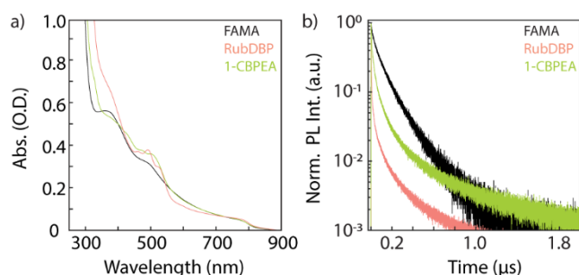
Figure 3: a) Absorption spectra for the FAMA perovskite thin film (black) and bilayer devices (RubDBP: pink, 1-CBPEA: green). b) Perovskite PL decays for the FAMA and bilayer devices under 780 nm excitation at an excitation density of 44.2 \text{ mW cm}^{-2} . A 780 nm notch filter and an 800 nm long pass filter were used to remove laser scatter and isolate the perovskite emission.
