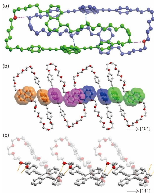
Fig. 2 Crystal structure of cyclophane 1 in the Cr_1 phase. Hydrogen atoms are omitted for clarity except for those involved in C-H...O and C-H... \pi interactions. (a) Dimer structure of cyclophane 1 . Blue and purple arrows correspond to C-H... \pi and C-H...O interactions, respectively. Each molecule is coloured green or blue except for oxygen atoms which interact with C-H bonds. (b) Adjacent luminophores form partially \pi -stacked structures in the plane parallel to (111). The \pi ... \pi -stacking between naphthalene rings and between anthracene rings is alternately arranged in the [-101] and [101] directions. Luminophores in the same molecules are depicted in the same colour. (c) Intermolecular C-H...O interactions along the [111] direction are depicted as orange-dotted lines, which occur between 2D assemblies of dimers parallel to the (111) plane.
