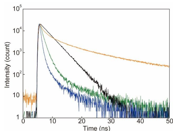
Fig. 8 Emission decay profiles of cyclophane 1 in dilute CHCl 3 solution (black), in the Cr 1
