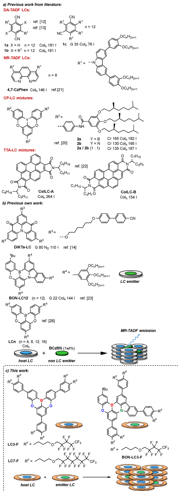
Fig. 1 Overview of literature-known TADF-LCs; (b) our previous work on MR-TADF LCs ( DiKTA-LC , BON-LC , LCn ); (c) our new strategy towards liquid crystalline emitter host mixtures features MR-TADF emission at room temperature.
