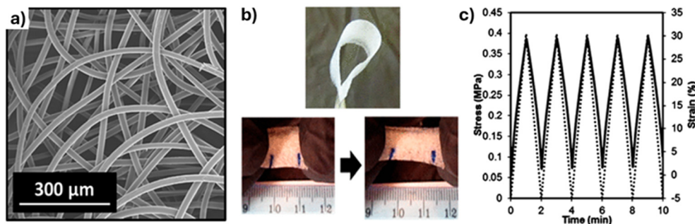
Fig. 4 Highly stretchable thiol-ene thermoset fibrous non-wovens: (a) SEM and (b) digital images of PTT/TVE non-woven mat showing its flexible and stretchable nature; (c) stress/strain cycling behavior (at 20\text{ }^{\circ}\text{C} , stress: dotted line, strain %: solid line). Figure adapted from ref. 39 with permission from American Chemical Society, Copyright © 2014.
