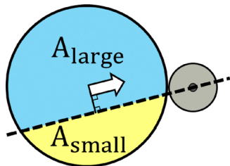
Fig. 3 Illustration of the definition of the symmetry parameter S . When a droplet first contacts an obstacle (shaded gray), a dividing line (dashed line) is drawn through the droplet to form two regions with areas A_{\text{large}} (shaded blue) and A_{\text{small}} (shaded yellow). The dividing line is parallel to the center of mass velocity vector of the droplet (large white arrow) and passes through the center of the obstacle.
