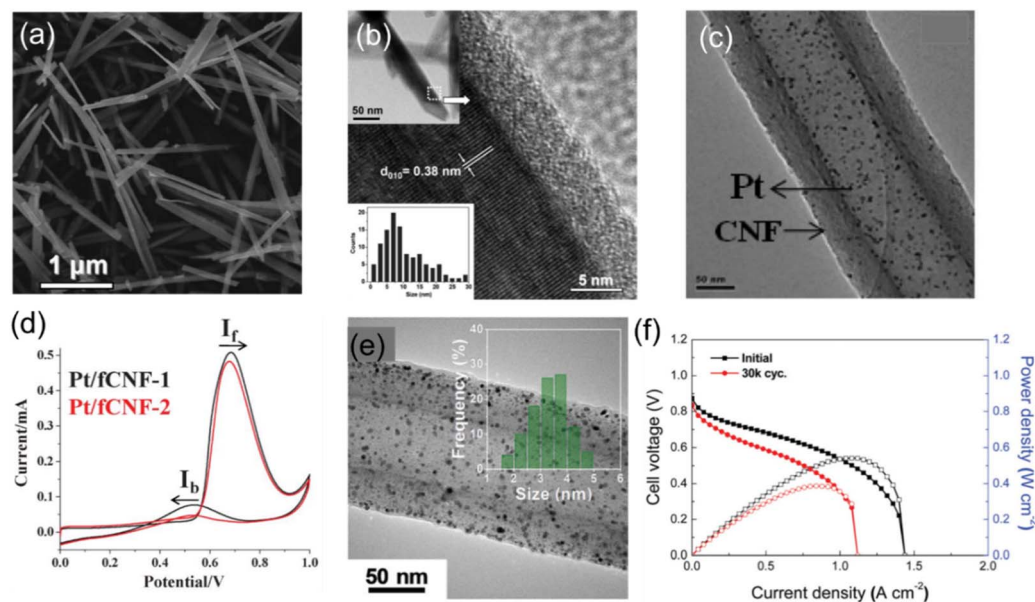
Fig. 11 (a) SEM image of TiO 2 nanofibers and (b) TEM images of TiO 2 /C. Upper inset: low-magnification TEM image of several fibers; lower inset: distribution of carbon thickness over different regions and fibers, (a and b) adopted from ref. 231, Copyright© Royal Society of Chemistry-(2012), (c) TEM image of Pt/fCNF-1 core-shell nanofibers, and (d) cyclic voltametric responses for methanol electro-oxidation by Pt/fCNF-1 (response after 60 min) and Pt/fCNF-2 (response after 63 min) modified electrodes (labelled) under acidic conditions (1 M methanol + 0.5 M H 2 SO 4 ) at a scan rate of 0.01 V vs. Ag/AgCl. (c and d) adopted from ref. 232, Copyright© Royal Society of Chemistry-(2013). (e) TEM images of Pt@CS/CNF600 core-shell nanofibers. (f) Polarization curves of (a) Pt/C, before and after 30 k AST cycles. Solid and open symbols represent the cell voltage and power density, respectively. (e and f) adopted from ref. 233, Copyright© Royal Society of Chemistry-(2019).
