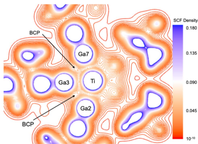
Fig. 2 SCF density plot along the Ti–Ga2–Ga3–Ga7 plane extracted from the QTAIM topological analysis, reflecting the Ga l –Ga l bond paths along which the Ga l –Ga l bond critical points (BCPs) are located.
