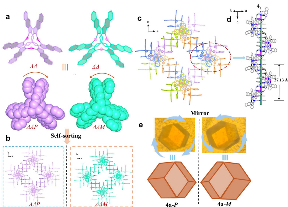
Fig. 3 Crystal structure of 4a . (a) \Delta\Delta - and \Delta\Delta -[ \text{Ag}_3\text{L}_4\text{L}_2 ] ^{3+} in 4a-P or 4a-M . (b) Narcissistic self-sorting of [ \text{Ag}_3\text{L}_4\text{L}_2 ] ^{3+} forming chiral structures of 4a-P and 4a-M . (c) Chiral srs network of 4a-P . (d) 4_1 \pi -stacked helical column along the c axis. (e) The photos of 4a-P/4a-M crystals.
