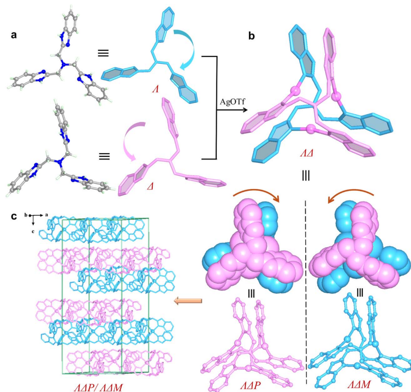
Fig. 1 Racemic crystal structure of 1. (a) \Delta - and \Delta -L 1 . (b) \Delta\Delta P - and \Delta\Delta M -[Ag 3 L 2 ] 3+ . (c) \Delta\Delta P -[Ag 3 L 2 ] 3+ and \Delta\Delta M -[Ag 3 L 2 ] 3+ align alternately along the c axis.
